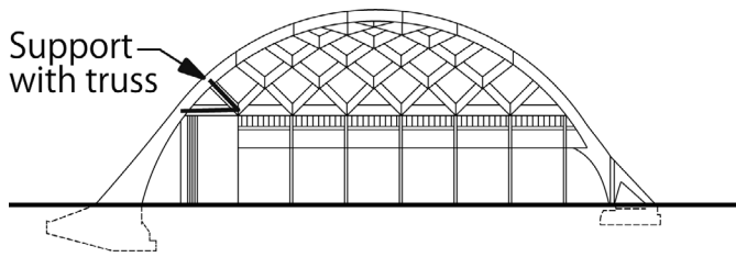
Figure 33. Cross section
