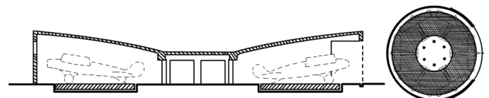
Figure 3. Section and plan of a hangar in RC shell (Patent) (1932)
