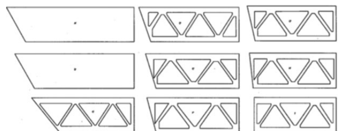
Figure 36. Rigid joint between the roof and the pillar
