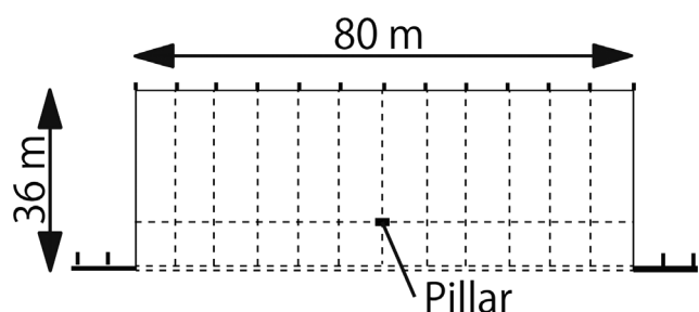
Figure 16. Plan for Ciampino Airport (Type A)
