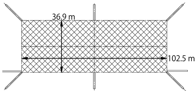
Figure 34. Plan of the hangar at Orbetello
