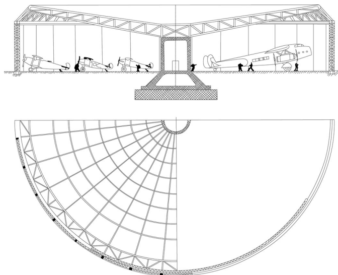
Figure 2. Section and plan of a circular hangar in steel
