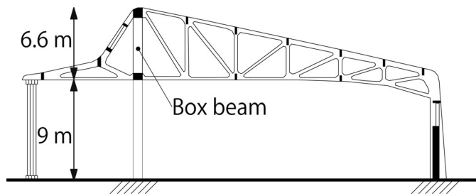
Figure 17. Cross section (Shorter side)
