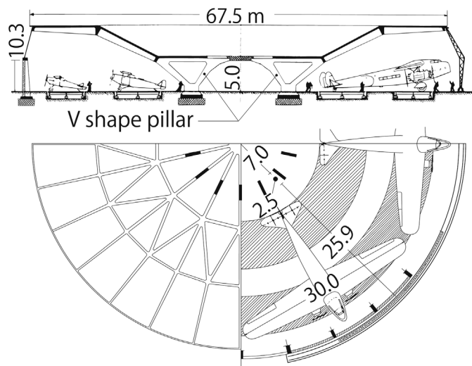
Figure 1. Section and plan of a circular hangar in reinforced concrete (RC)
