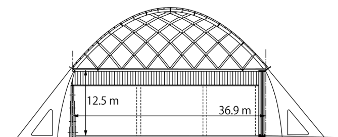
Figure 35. Cross section
