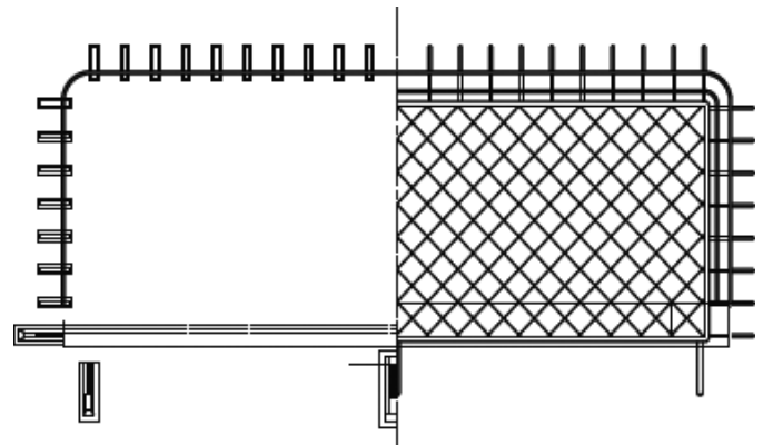
Figure 28. Plan of the hangar for Ciampino Airport (Plan D)
