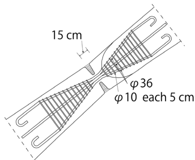
Figure 31. Bar arrangement of the arch
