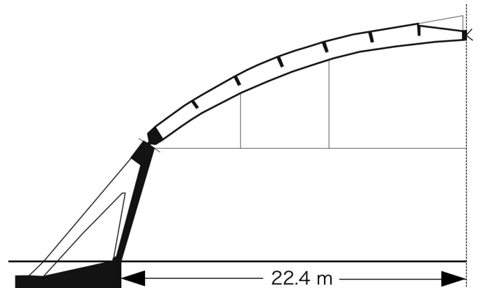
Figure 27. Cross section of hangar for Ciampino Airport (Plan C)
