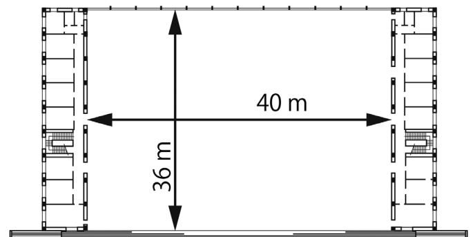
Figure 11. Plan of a hangar for an Italian Air Force platoon
