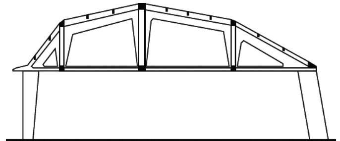
Figure 22. Cross section of hangar for Ciampino Airport (Type B)
